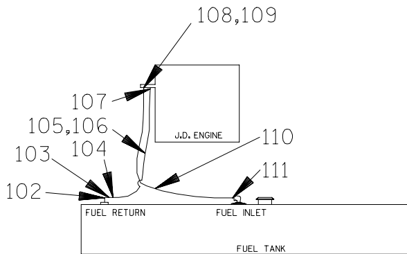
FUEL LINE ASSEMBLY
