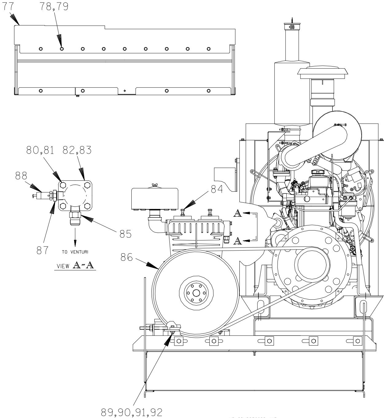
AIR COMPRESSOR AND ENGINE ASSEMBLY END VIEW
