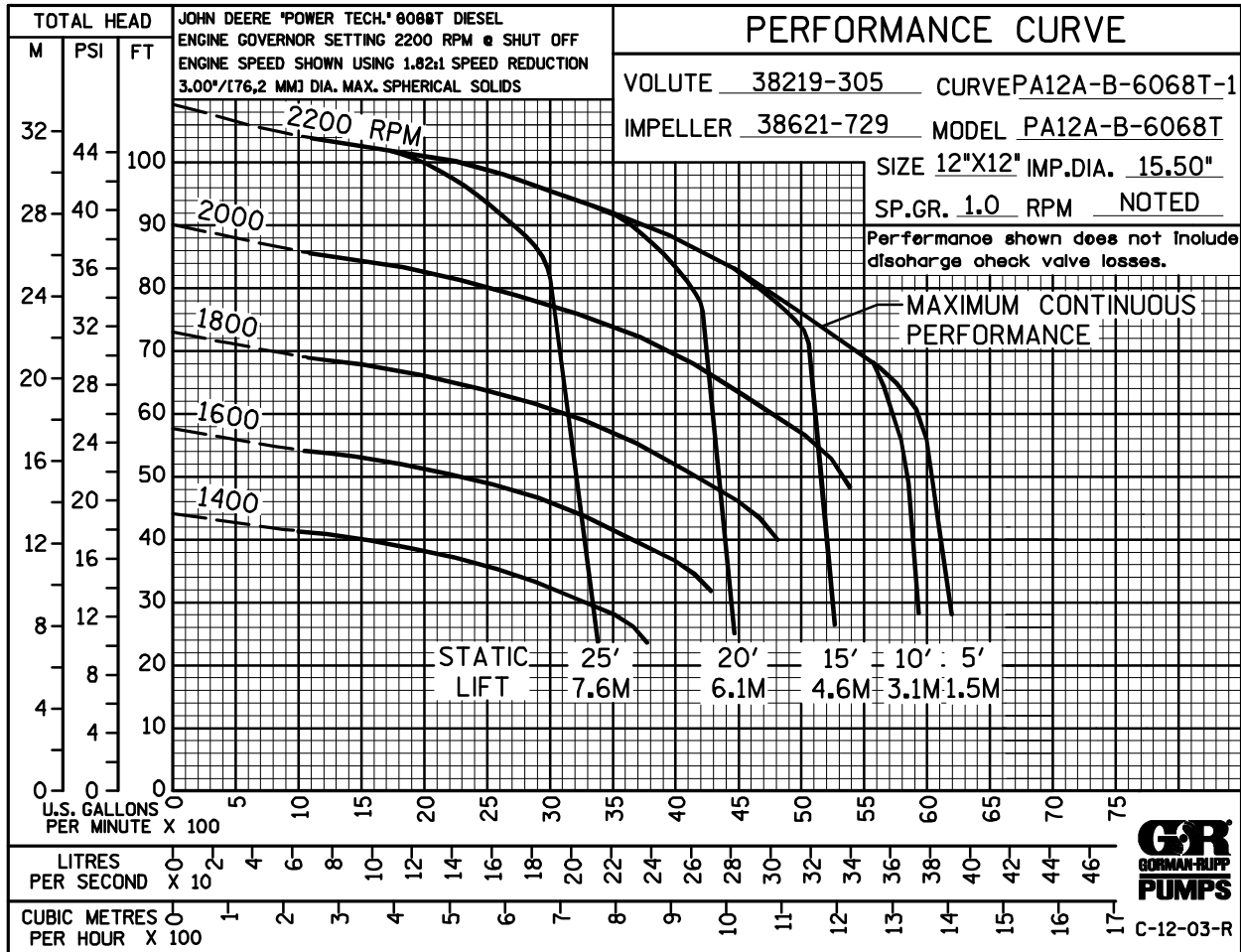
Performance Curve – Model PA12A60-B-6068T
