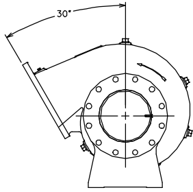
VOLUTE ORIENTATION AS VIEWED FROM SUCTION PORT. USE FOR MODEL PABA60-6068T SU ONLY.
