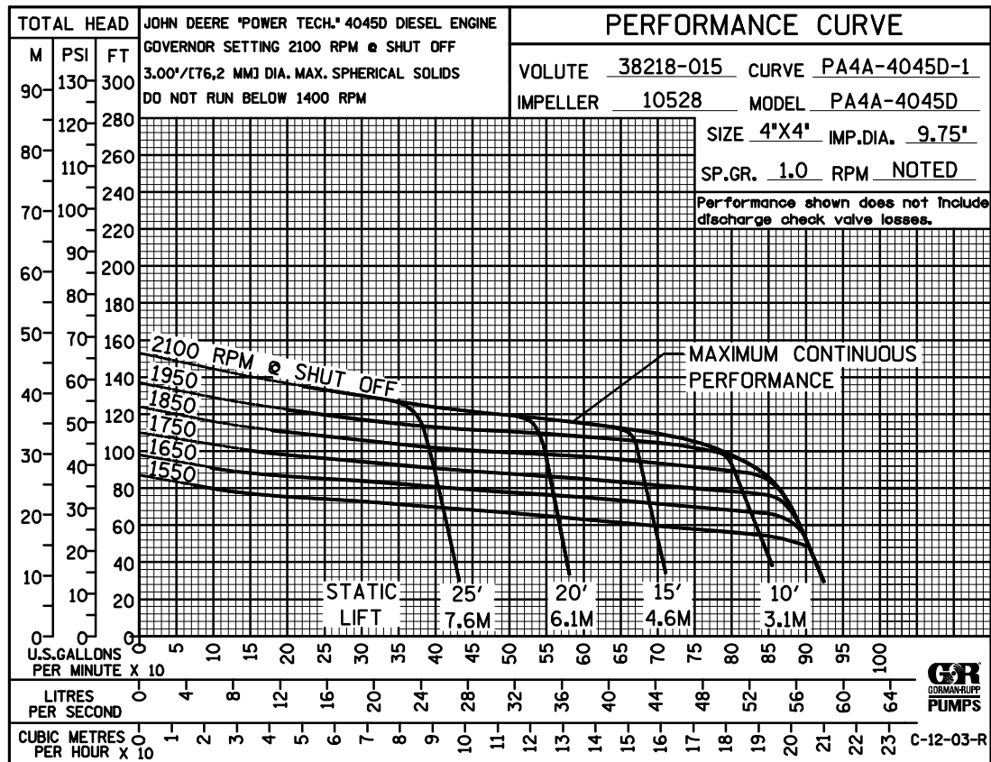
Performance Curve – Model PA4A60–4045D
