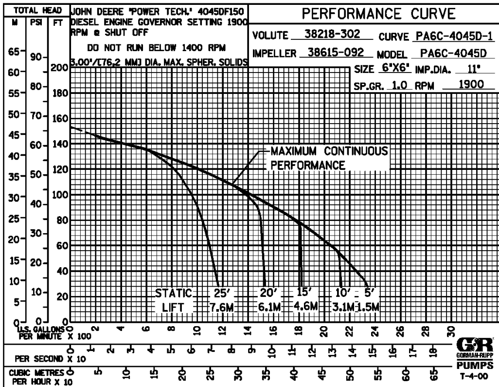
Performance Curve – Model PA6C60-4045D-A
