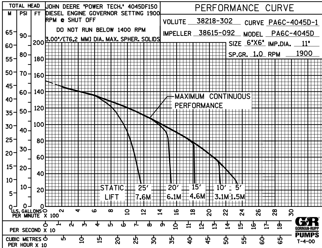
Performance Curve – Model PA6C60-4045D
