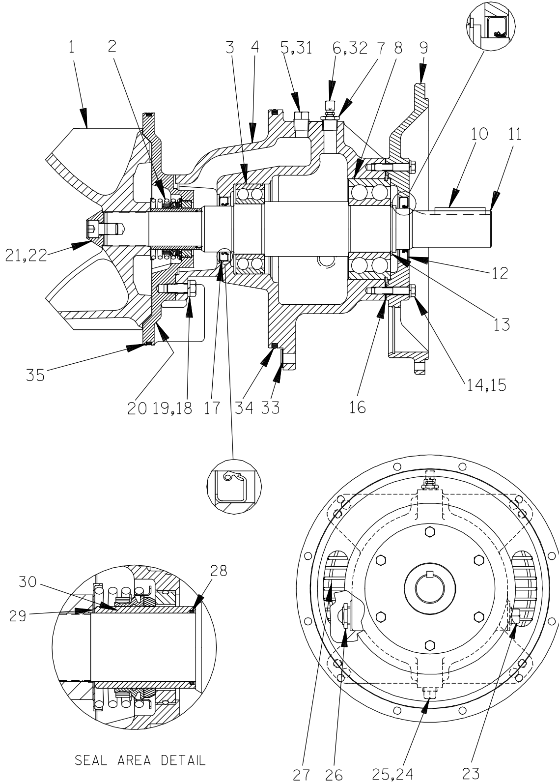
DRIVE END VIEW
