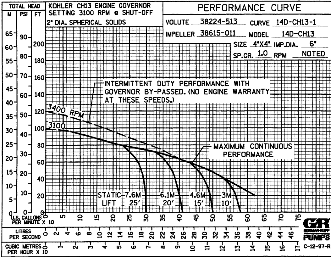
Performance Curve – Models 14D1-CH13 And 14D1-CH13 S/G
