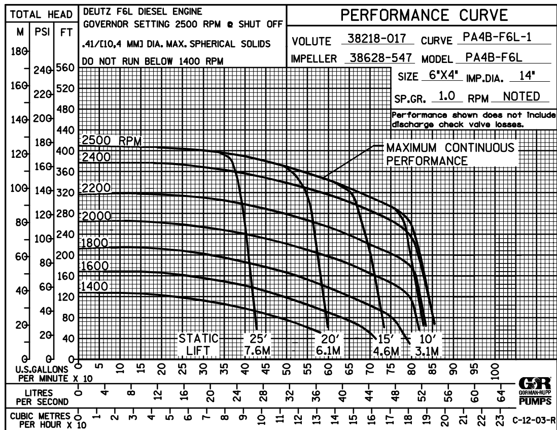
Performance Curve – Model PA4B60–F6L
