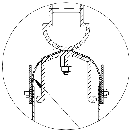
VALVE DETAIL
