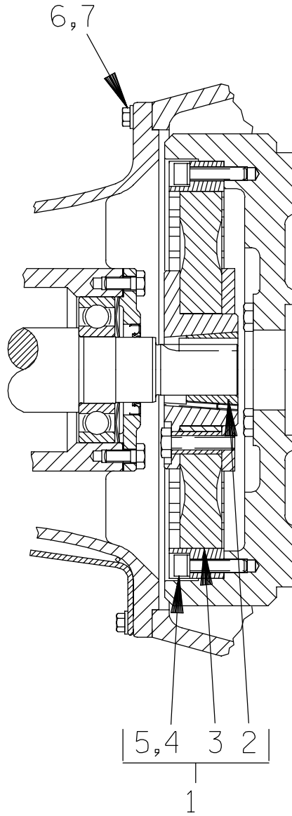
44162-119 Drive Assembly
