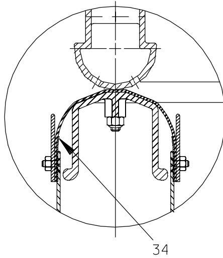
VALVE DETAIL
