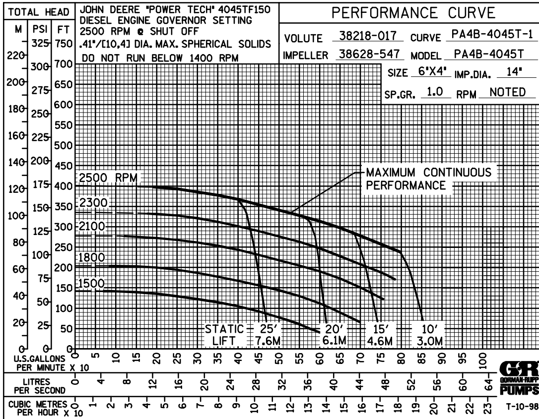
Performance Curve – Model PA4B60-4045T
