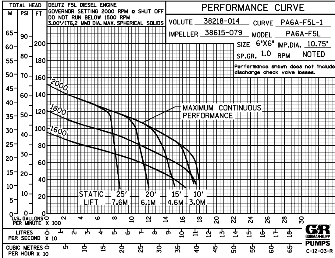
Performance Curve – Model PA6A60-F5L
