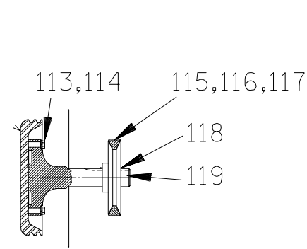
FRONT ENGINE CRANKSHAFT EXTENSION ASS'Y.
