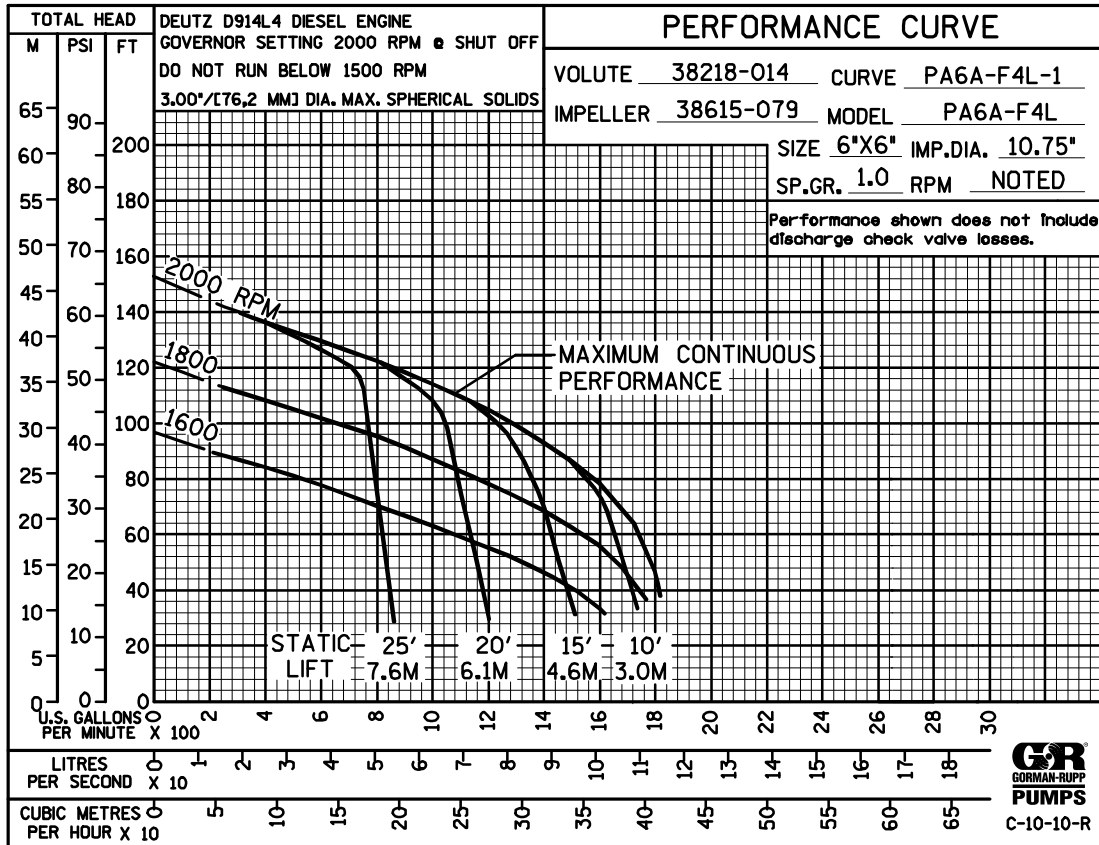
Performance Curve – Model PA6A60–F4L
