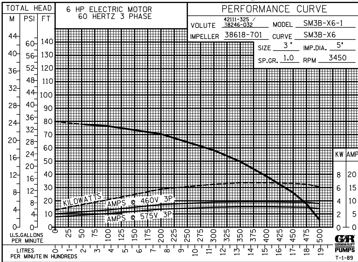
Performance Curve – Model SM3B65-X6 460/575/3
