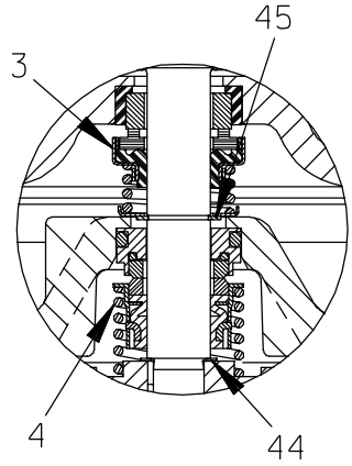
SEAL AREA DETAIL
