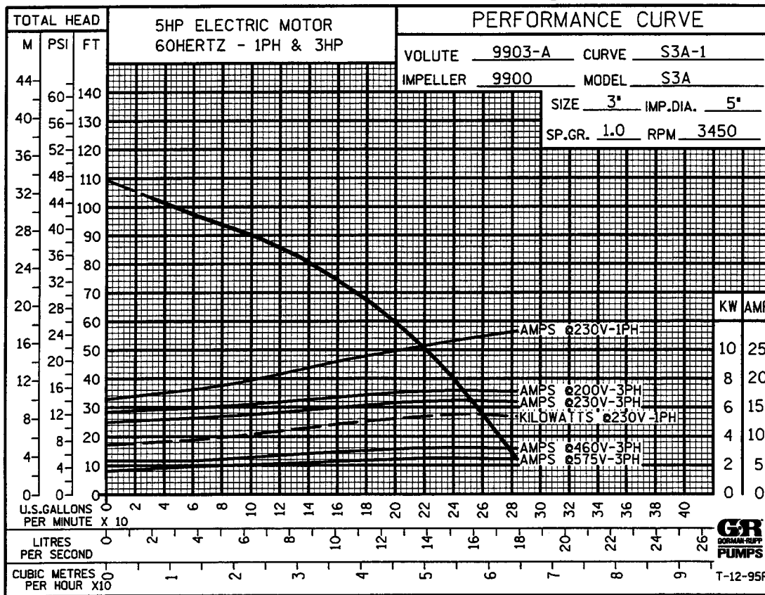
Performance Curve – Model S3A1-230V 1P
