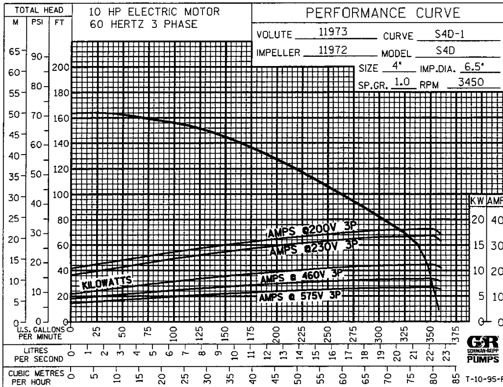
Performance Curve – Model S4D1 460V 3P
