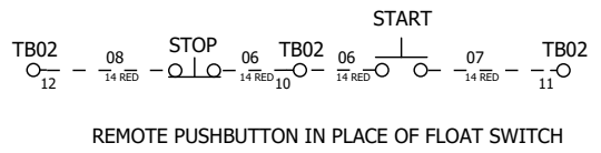
REMOTE PUSHBUTTON IN PLACE OF FLOAT SWITCH
