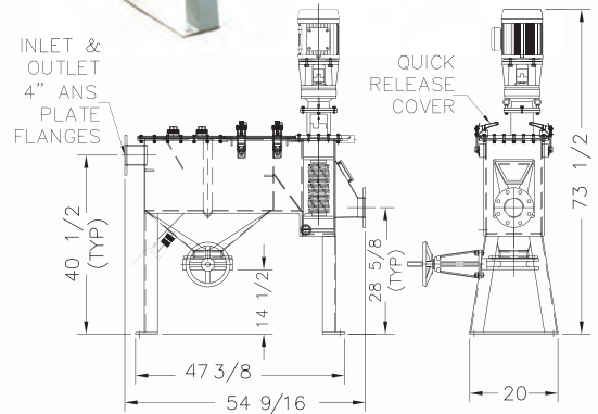
CUTTER CONFIGURATIONS
