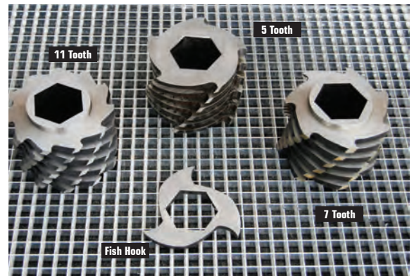
CUTTER CONFIGURATIONS
