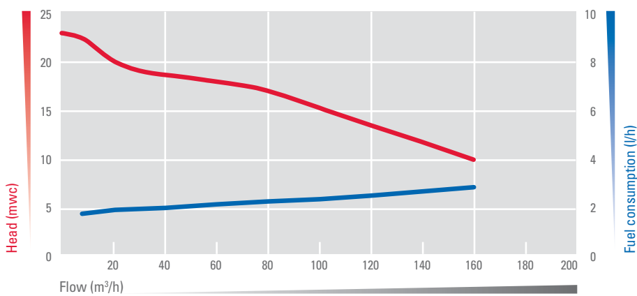
PA4-160 performance
