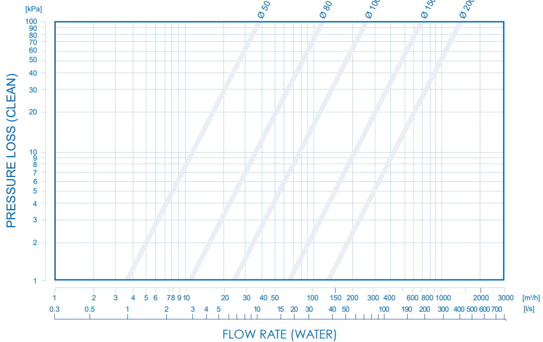
BASKET STRAINER PRESSURE LOSS CHART
